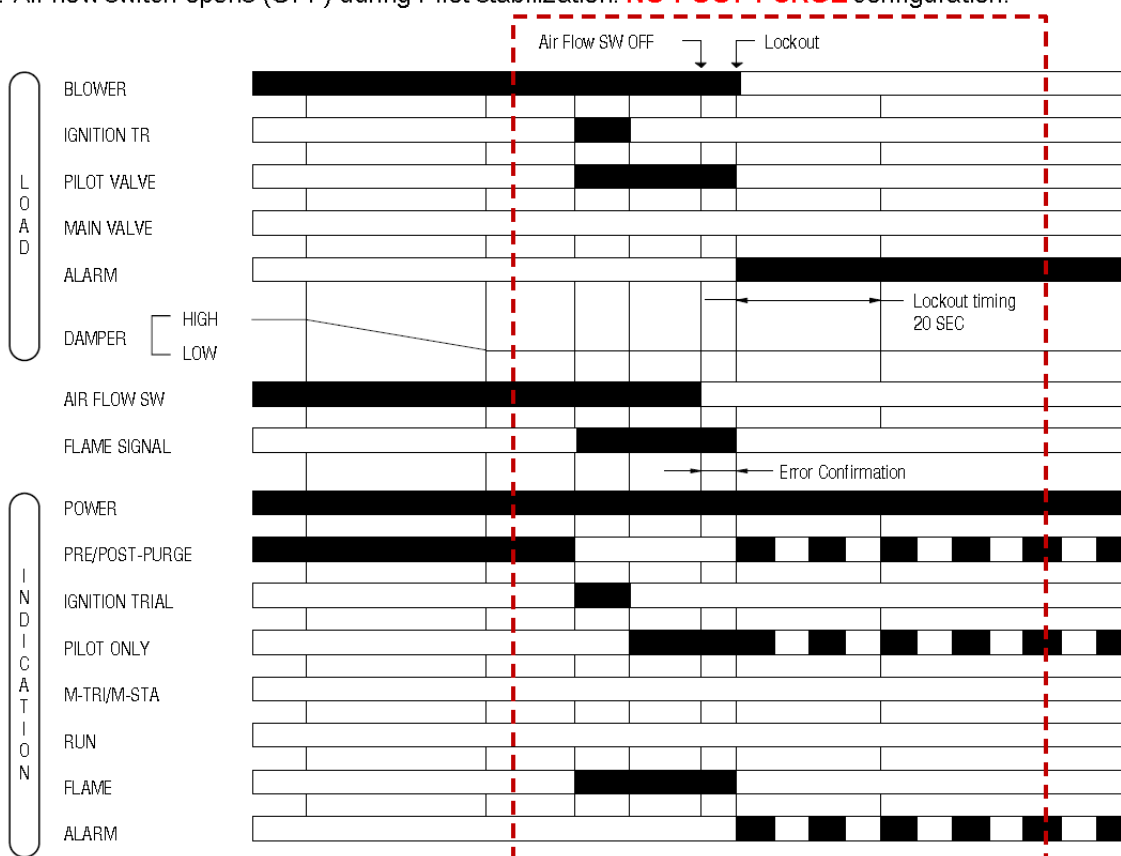
Fig 13b. Air flow switch opens (OFF) during Pilot stabilization: NO-POST-PURGE configuration.
