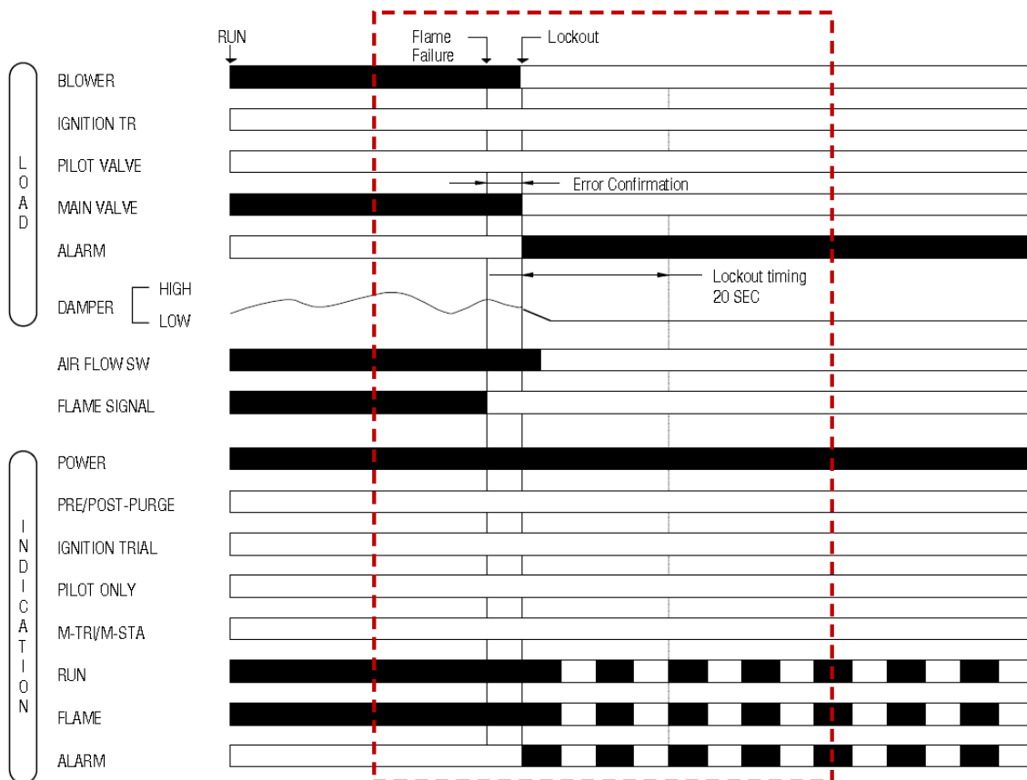
Fig 7b. Flame failure during run period: NO-POST-PURGE configuration.
