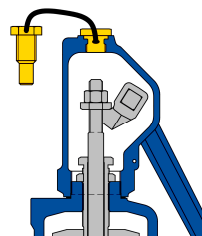
Type with test gag
