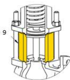
Type with insert 613, 673
