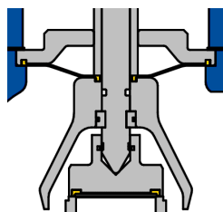
Type with membrane (01-4)
