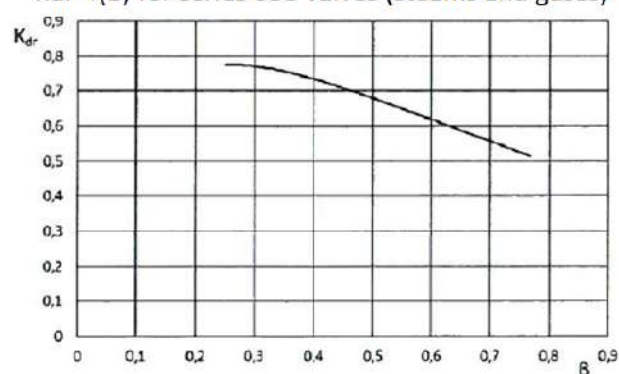
K dr =f(b) for series 630 valves (steams and gases)
