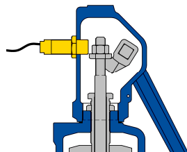
Type with inductive sensor
