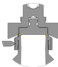
Type with stellited disc
