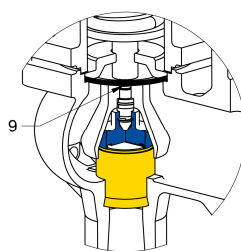
630 Type: 01 Sealing -4
