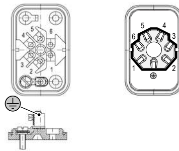
Fig. 5: Cable socket / plug
