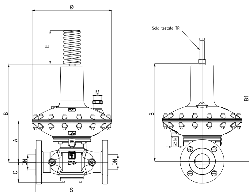
Figure 8 Dival 600 dimensions
